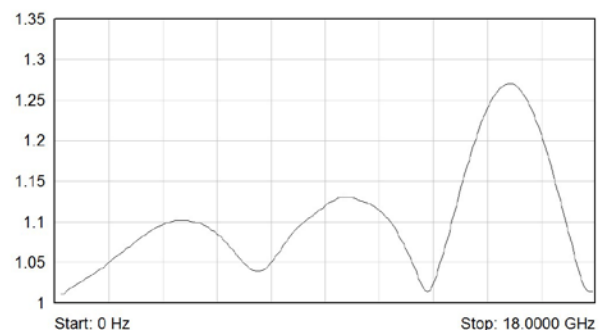
Typical VSWR Plot for 18 GHz Terminated Versions
