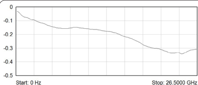
Typical Insertion Loss (dB) Plot for 26.5 GHz Underterminated Versions
