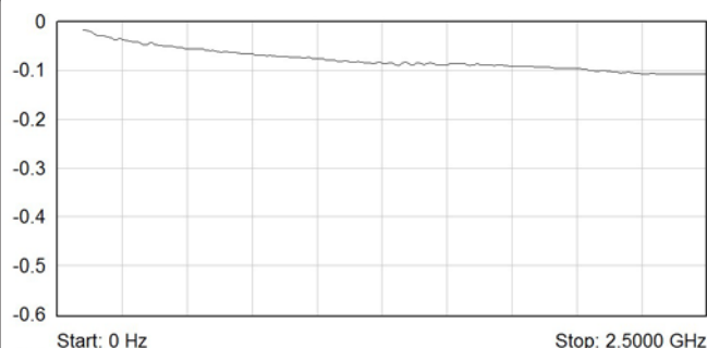
Typical Insertion Loss (dB) Plot for 2.5 GHz 75 \Omega Versions
