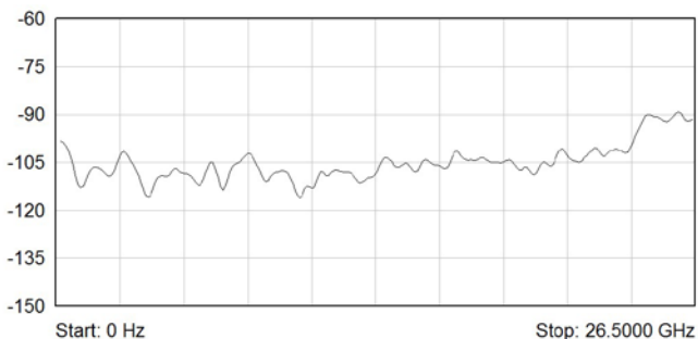
Typical Isolation (dB) Plot for 26.5 GHz Underterminated Versions
