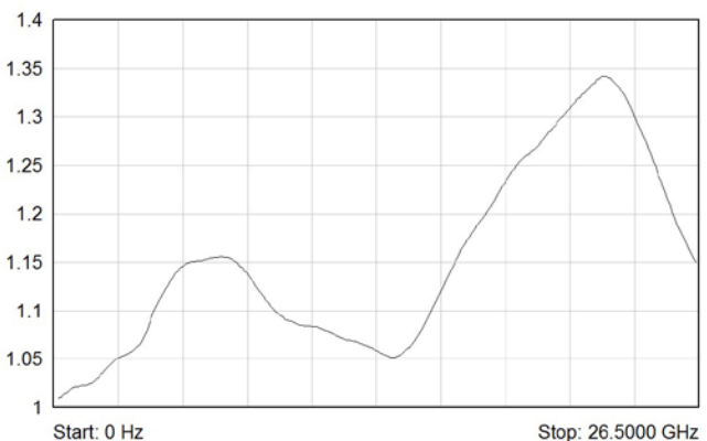
Typical VSWR Plot for 26.5 GHz Underterminated Versions
